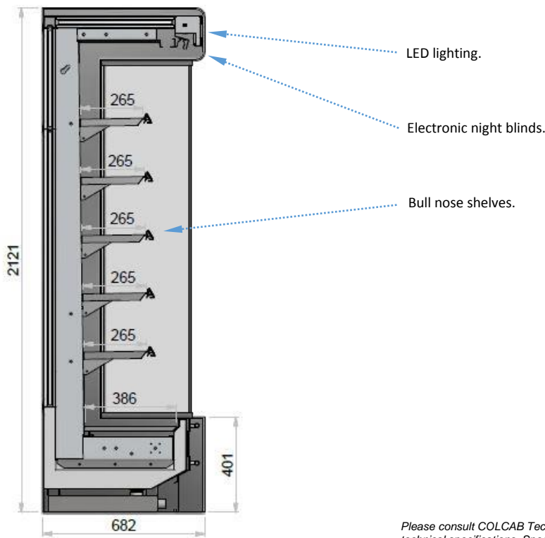
NARROW UPRIGHT CHILLED MERCHANDISER
