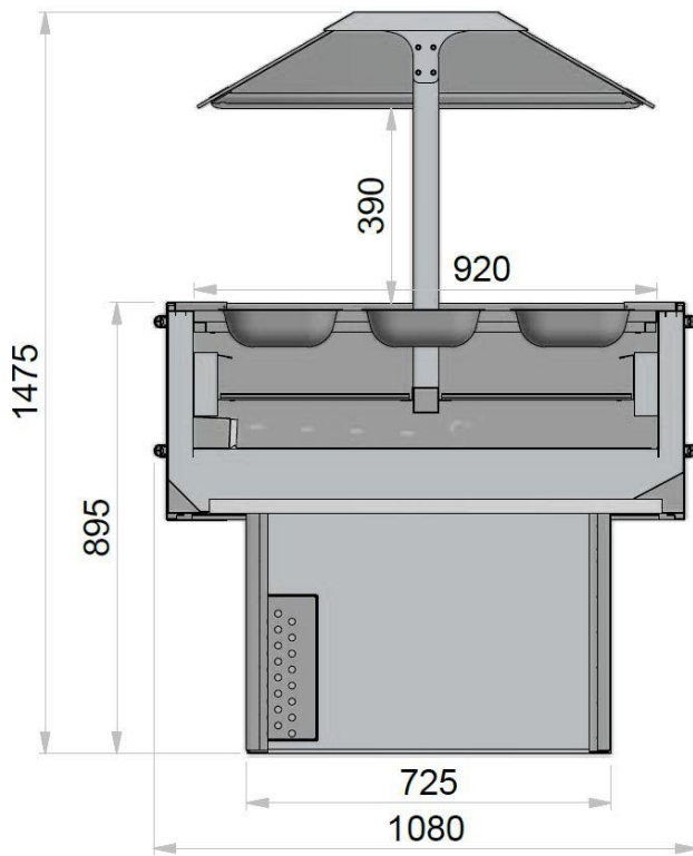
RECTANGULAR SALAD MERCHANDISER
